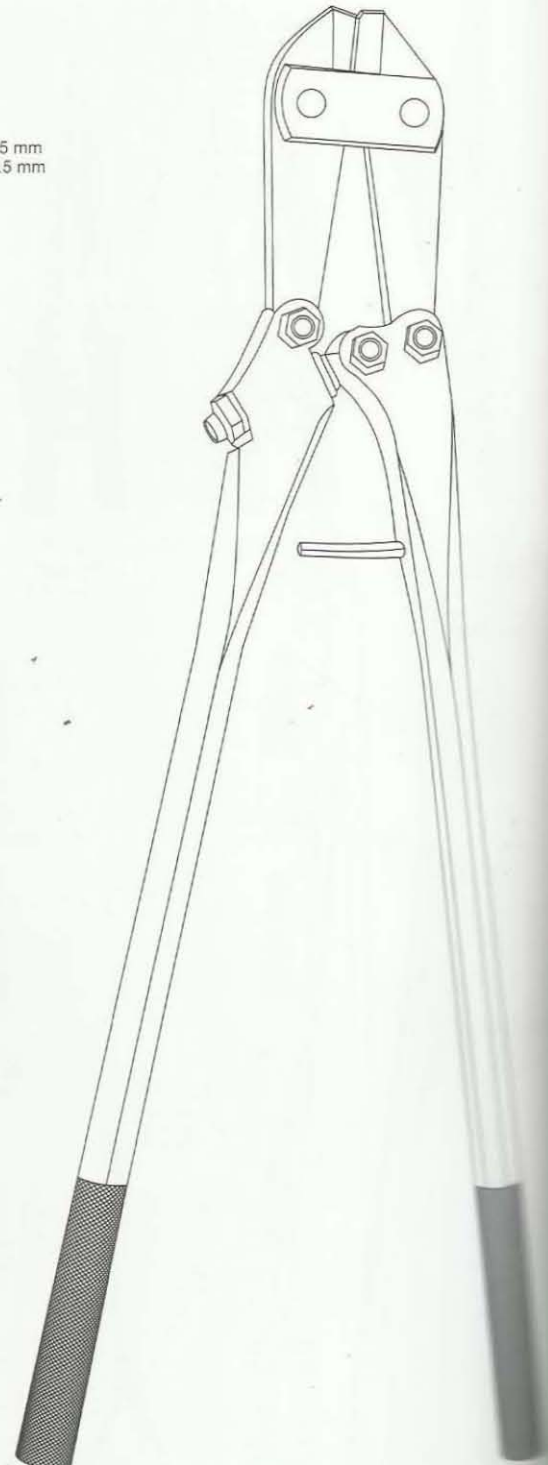
TC wire cutter For wire 90-463 38.5 cm / 15" 5 mm 90-464 45 cm / 17 3/4" 6 mm 90-465 56 cm / 22" 7.5 mm
