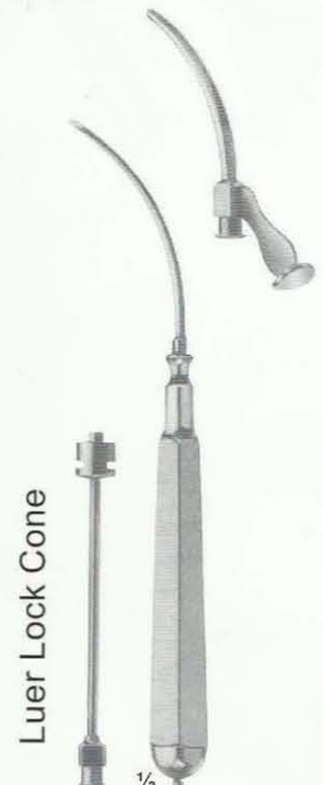
15-200 - 203 Inside diam Outside diam 15-200 2,2 mm 3,0 mm 15-201 3,0 mm 4,0 mm 15-202 4,0 mm 5,0 mm 15-203 5,0 mm 6,0 mm for abdominal puncture, with stop-cock and lateral drain
