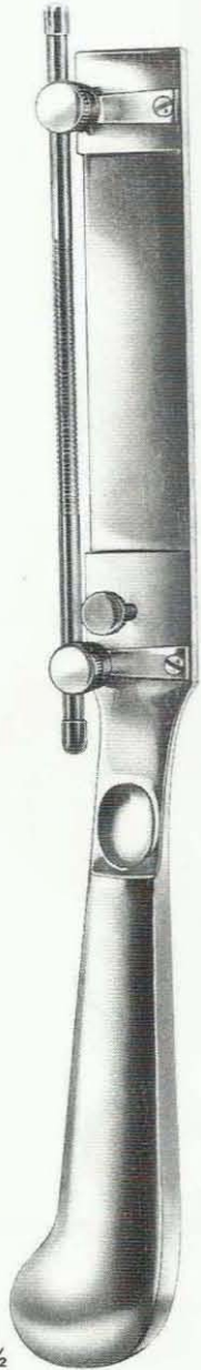
06-202 SCHINK Size: 310 mm Complete with 2 skin fixing plates and 1 blade. Adjustable from 0.1 to 2.0mm
